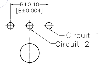
2-3 Circuit PCB LAYOUT
