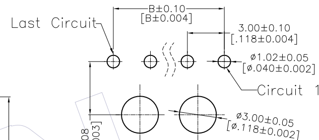
4-12 Circuit PCB LAYOUT
