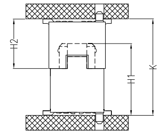
MATED DRAWING(REF.)
